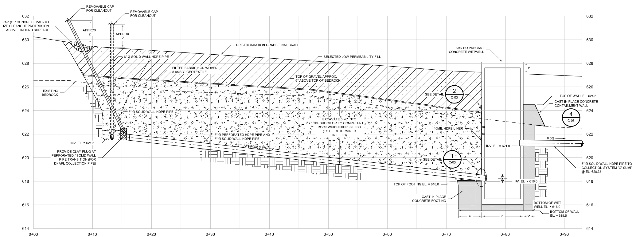
SECTION B HOR. 1" = 5' VER. 1" = 2.5'
