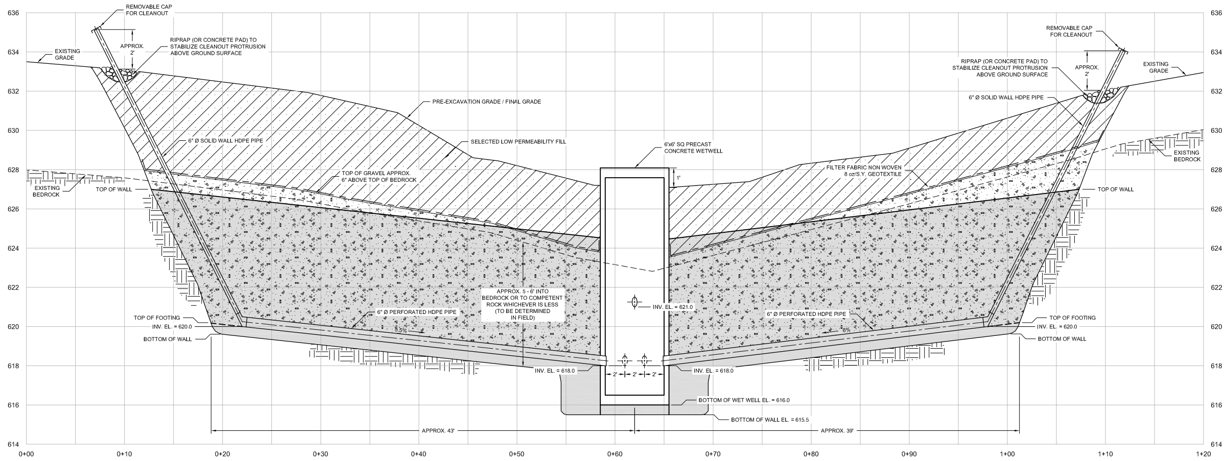
SECTION A HOR. 1" = 5' VER. 1" = 2.5'
